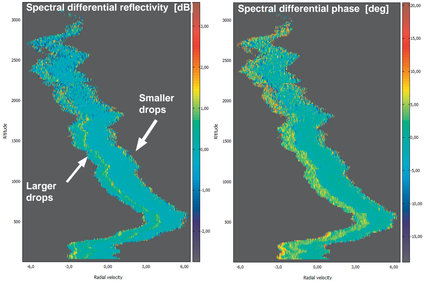
Fig. 13. Spectral polarimetric observations at 30 deg elevation in the STSR-mode. Spectral differential reflectivity and spectral differential phase vertical profiles. Measurements were taken at the RPG site, Meckenheim, Germany.
