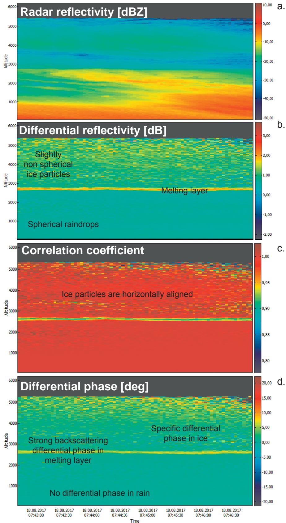
Fig. 12. Example of polarimetric observations in the STSR-mode. Time-height cross-sections of the radar reflectivity (a.), differential reflectivity (b.), correlation coefficient (c.), and differential phase shift (d.). Observations were made at 30 deg elevation angle. Measurements were taken at the RPG site, Meckenheim, Germany.
