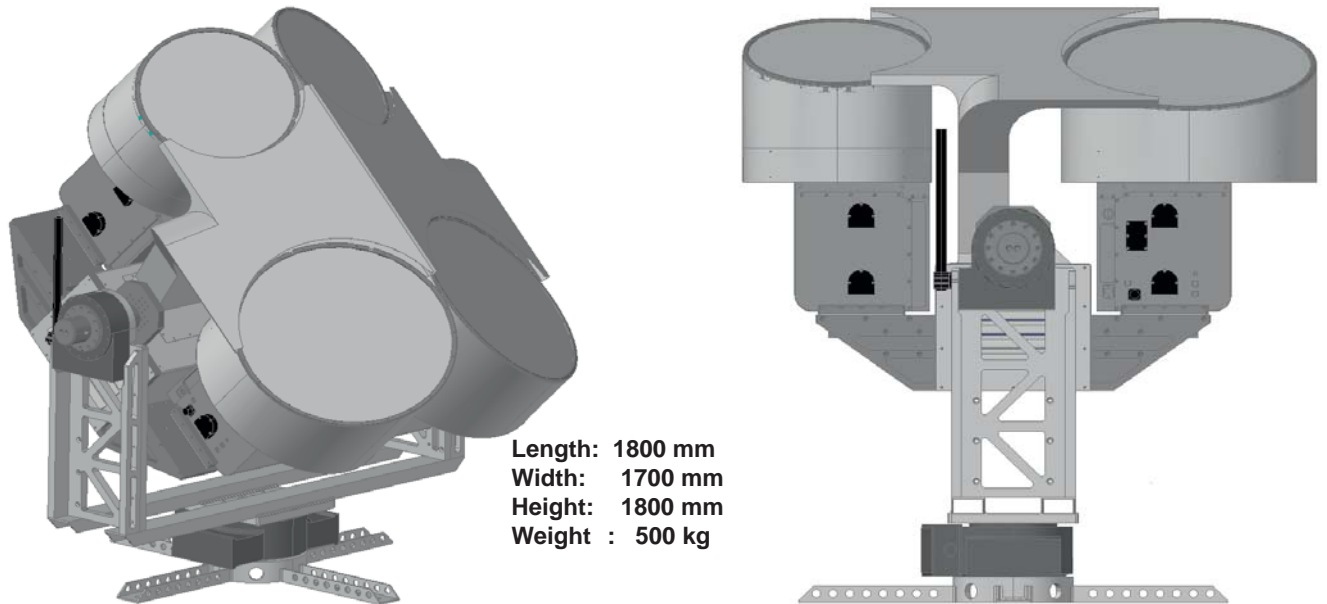
Fig. 14. Design of the dual wavelength radar system.
