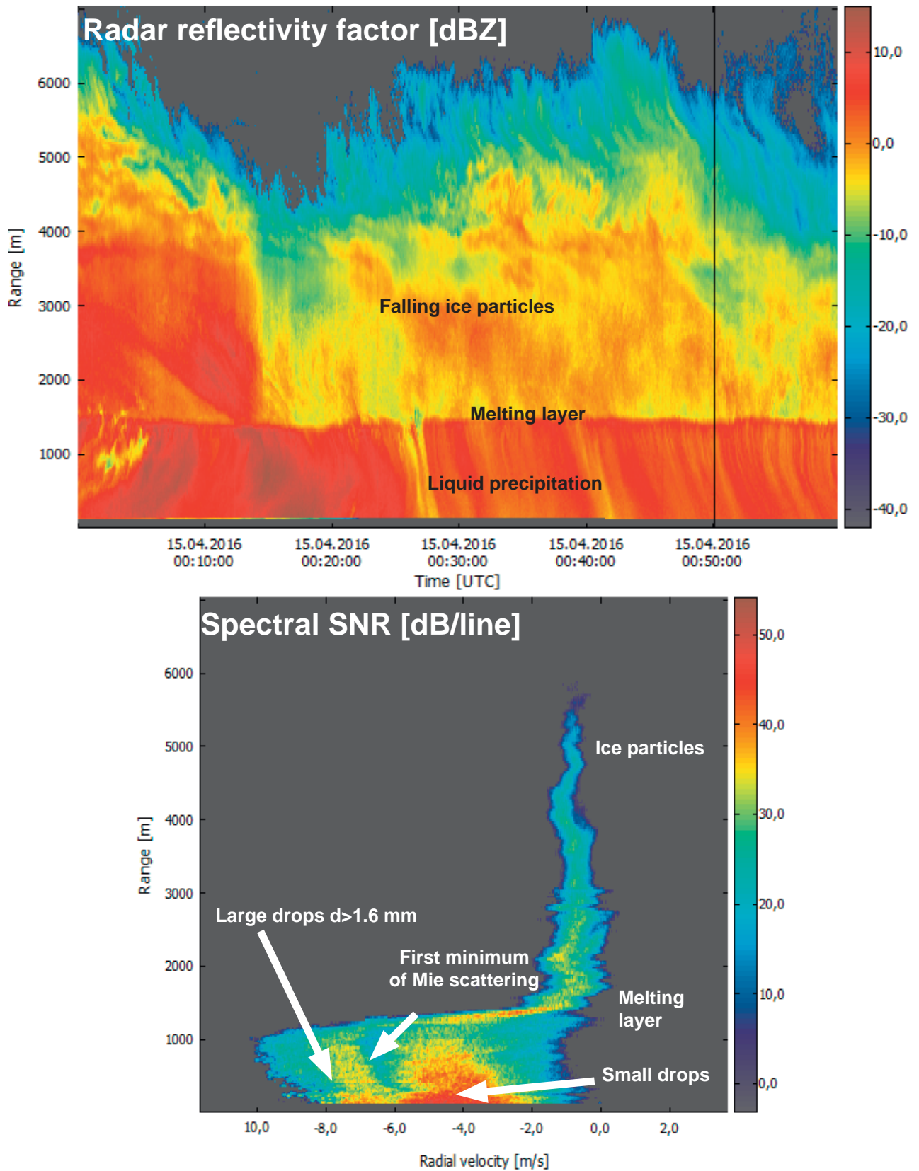
Fig. 7. The time range cross section of the radar reflectivity factor (upper panel) and the vertical profile of Doppler spectra for a cloud system observed on 15 April 2016 at the RPG site, Meckenheim, Germany. The vertical black line indicates the time sample corresponding to the Doppler spectrum profile.
