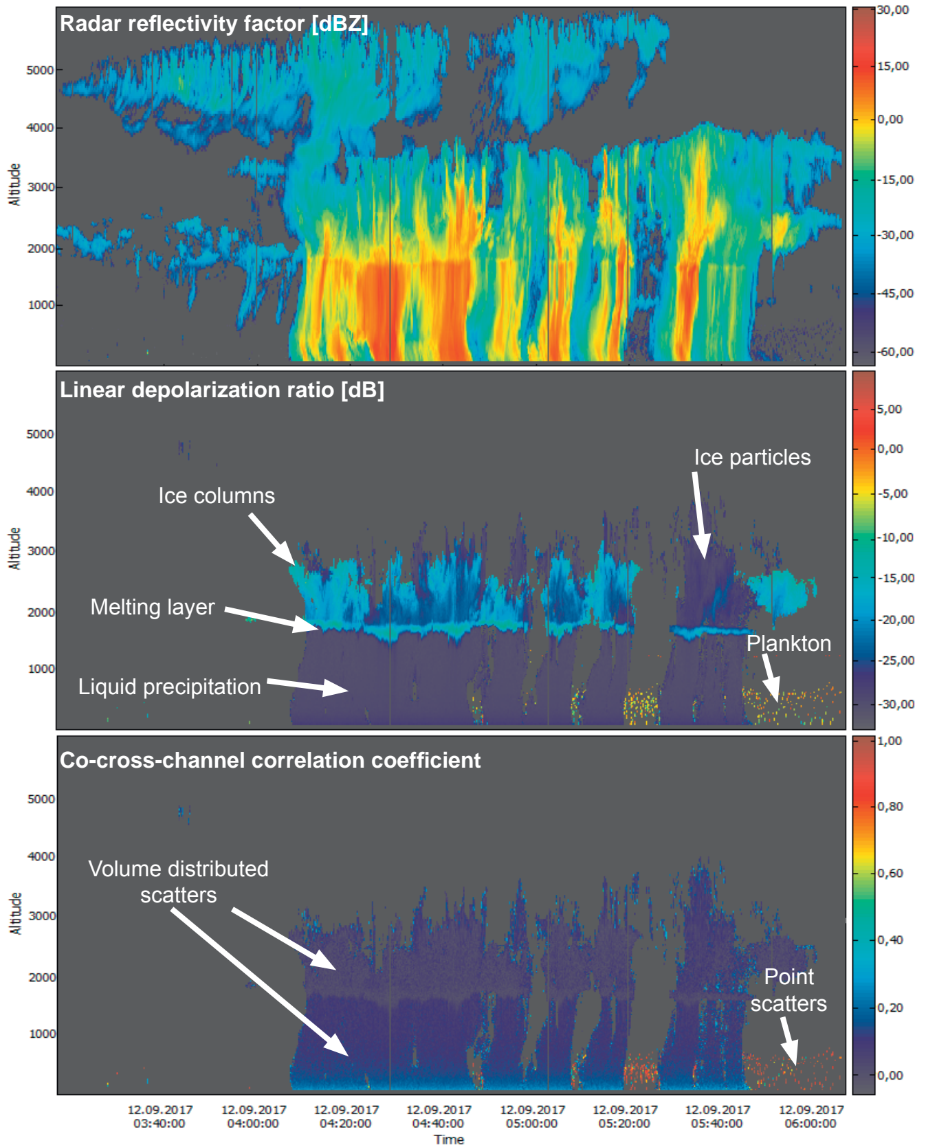
Fig. 11. Example of polarimetric observations in the LDR-mode. Time-height cross-sections of the radar reflectivity (upper panel), linear depolarization ratio (middle panel), and co-cross-channel-correlation coefficient (lower panel). During the measurements the radar was pointed vertically. Measurements were taken at the RPG site, Meckenheim, Germany.
