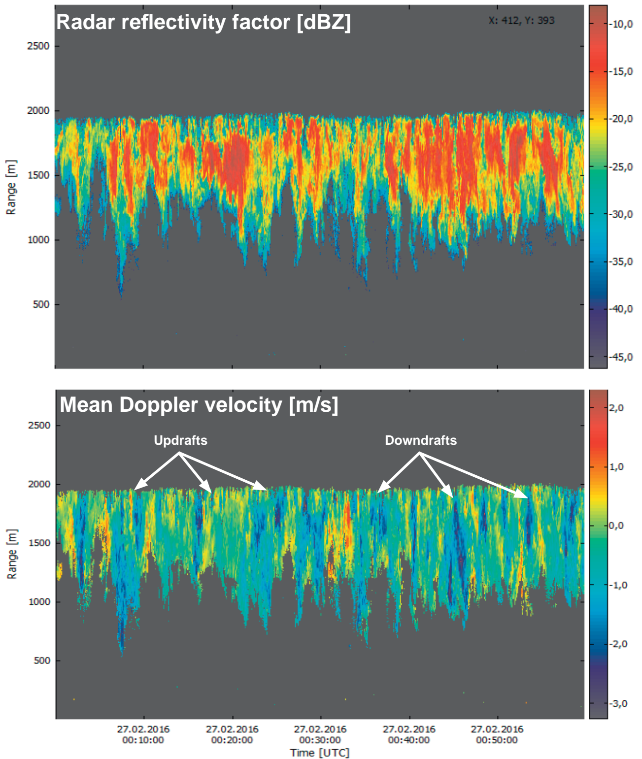
Fig. 5. The time range cross sections of the radar reflectivity factor (upper panel) and the mean Doppler velocity. The measurements were taken on 27 February 2016 at the RPG site, Meckenheim, Germany.
