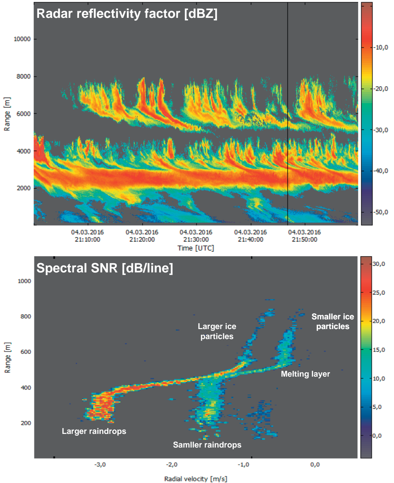
Fig. 6. The time range cross section of the radar reflectivity factor (upper panel) and the vertical profile of Doppler spectra for a cloud system observed on 4 March 2016 at the RPG site, Meckenheim, Germany. The vertical black line indicates the time sample corresponding to the Doppler spectrum profile.
