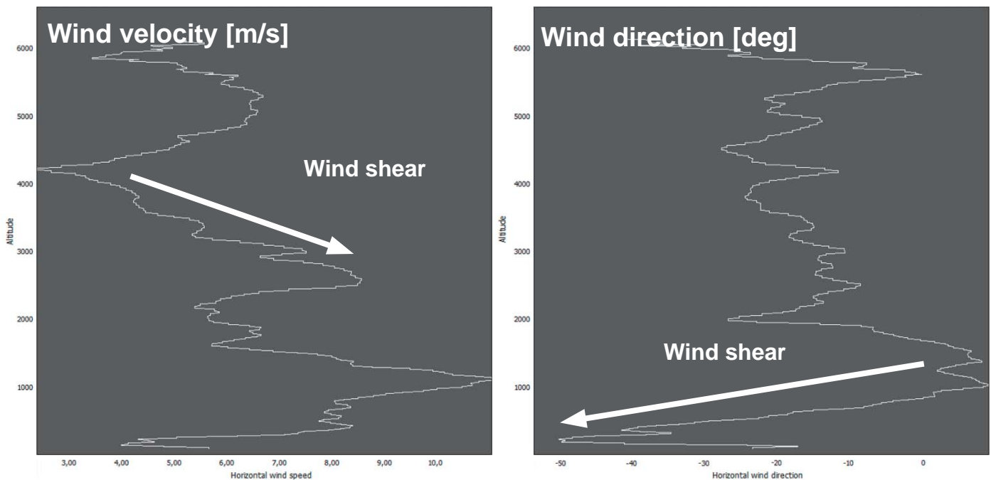
Fig. 10. Example of the wind retrieval corresponding to the measurements from Fig.10.
