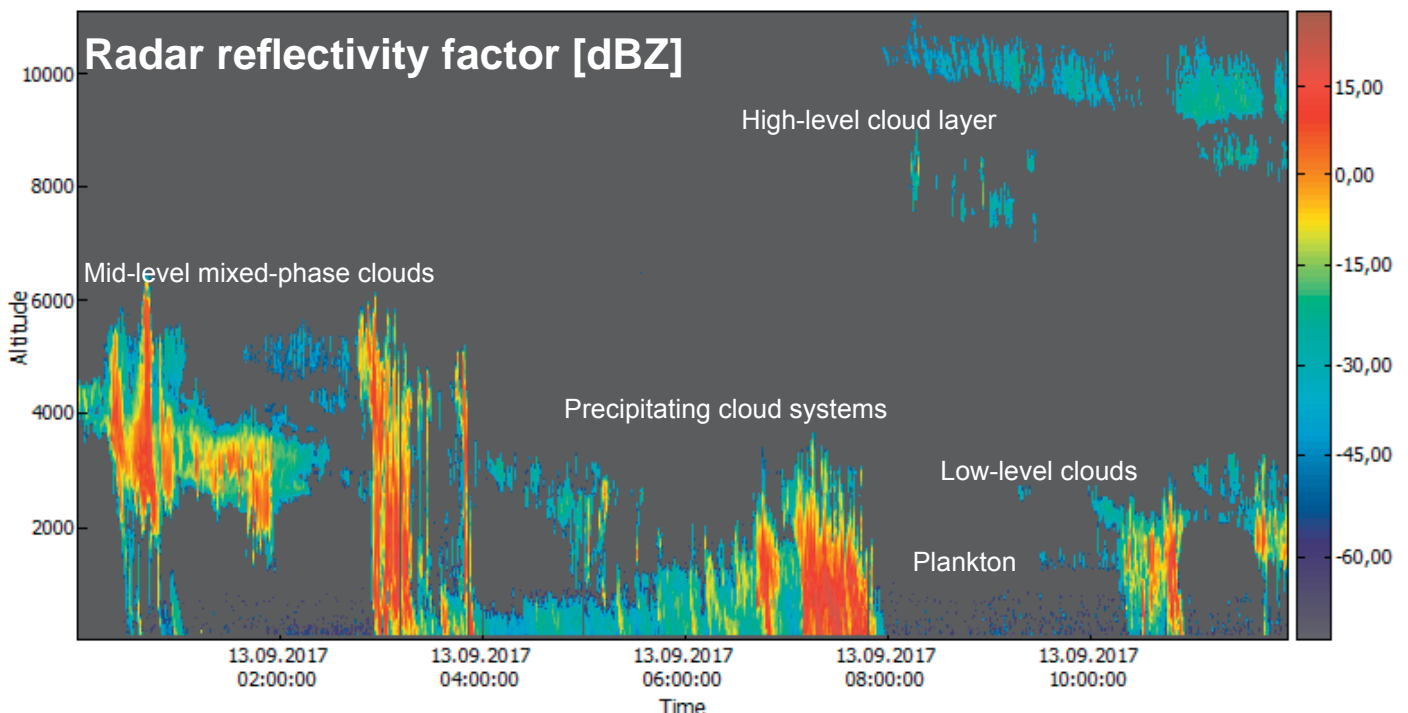
Fig. 3. The time-range cross section of the radar reflectivity factor. The measurements were taken on 13 Sep 2017 at the RPG site, Meckenheim, Germany
