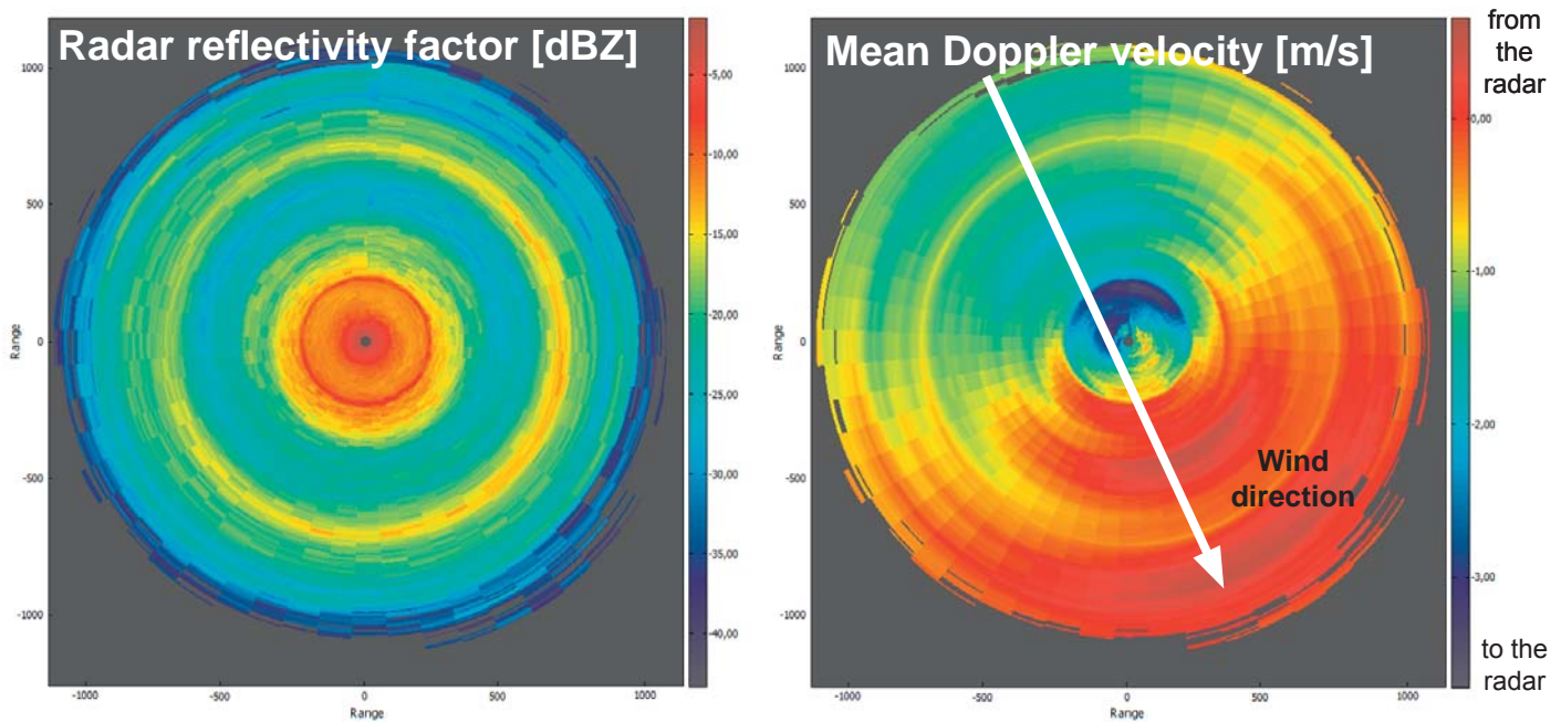
Fig. 9. Example of azimuthal scanning observations. Radar reflectivity factor (left panel) and mean radial Doppler velocity (right panel). The measurements were performed at the 80 deg elevation angle.
