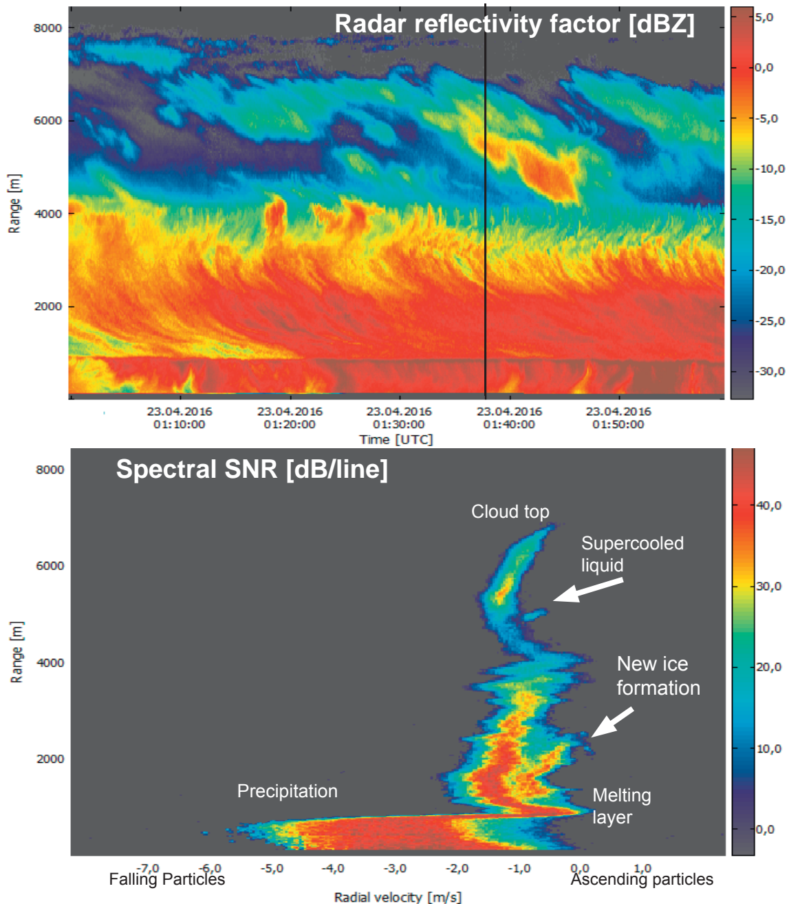
Fig. 4. The time range cross section of the radar reflectivity factor (upper panel) and the vertical profile of Doppler spectra for a deep precipitating cloud system observed on 23 Apr 2016 at the RPG site, Meckenheim, Germany. The vertical black line indicates the time sample corresponding to the Doppler spectrum profile.
